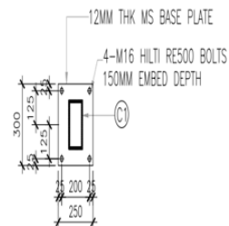
BASE PLATE-FOR RHS-(150X100X5.0)-COLUMN
